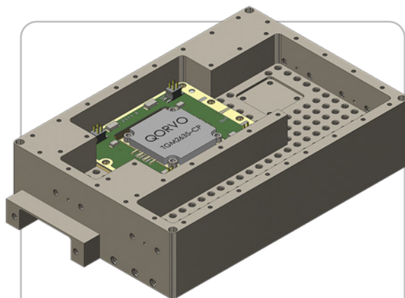
2. X-MWblock Drop-In on Copper Base and Heatspreader
