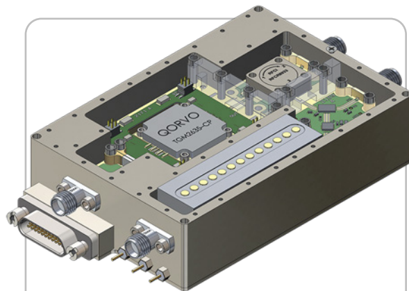
5. X-MWblock Drop-In Integrated with Additional X-MWblocks in Final Integrated Microwave Assembly
