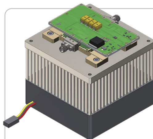
3. X-MWblock Drop-In on Heatsink Fan Assembly with Plug-In Pulse Circuit
